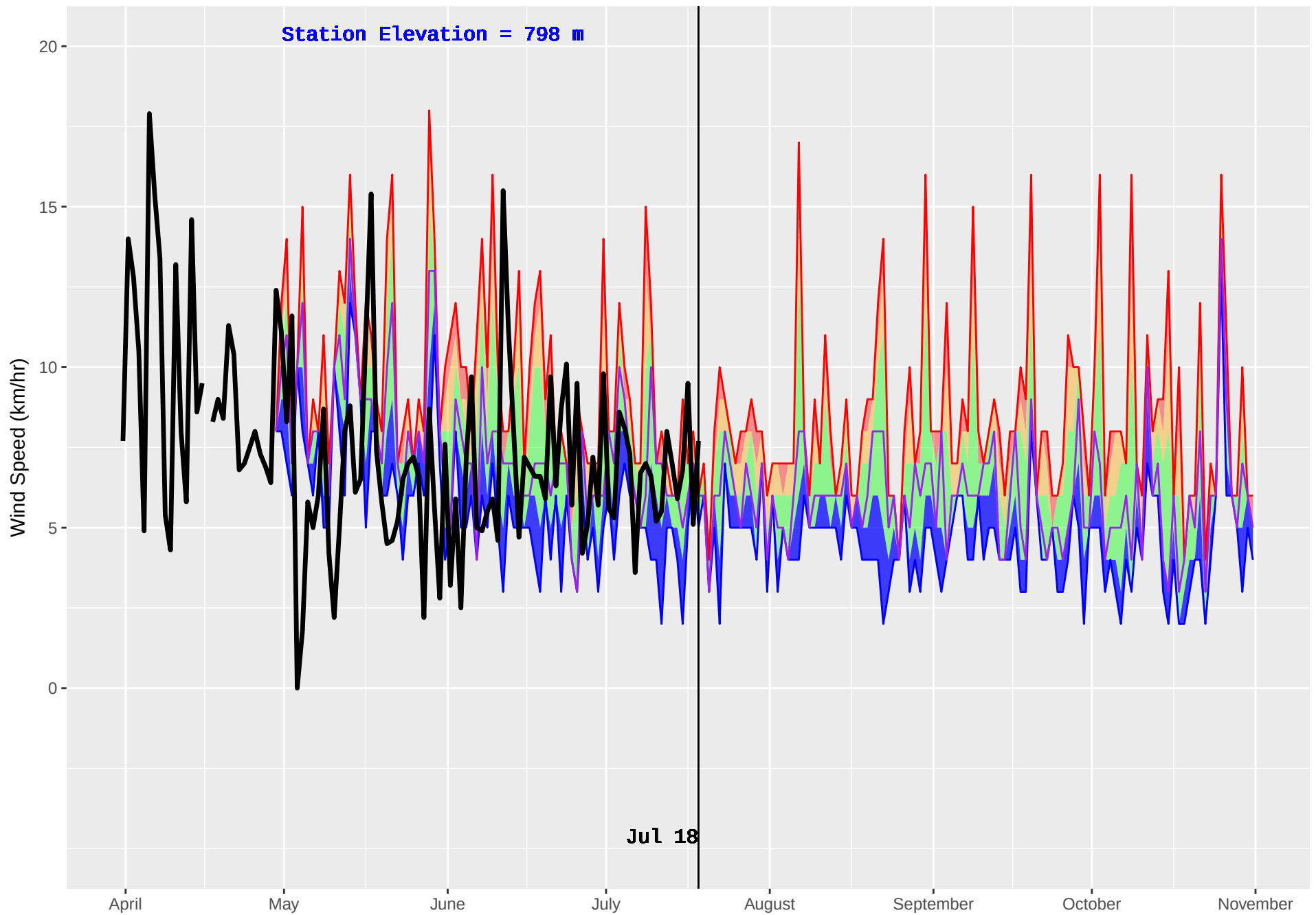
SEVEREID (1165) : Historical (2014–2016) and Current (2018) Daily Wind Speed
